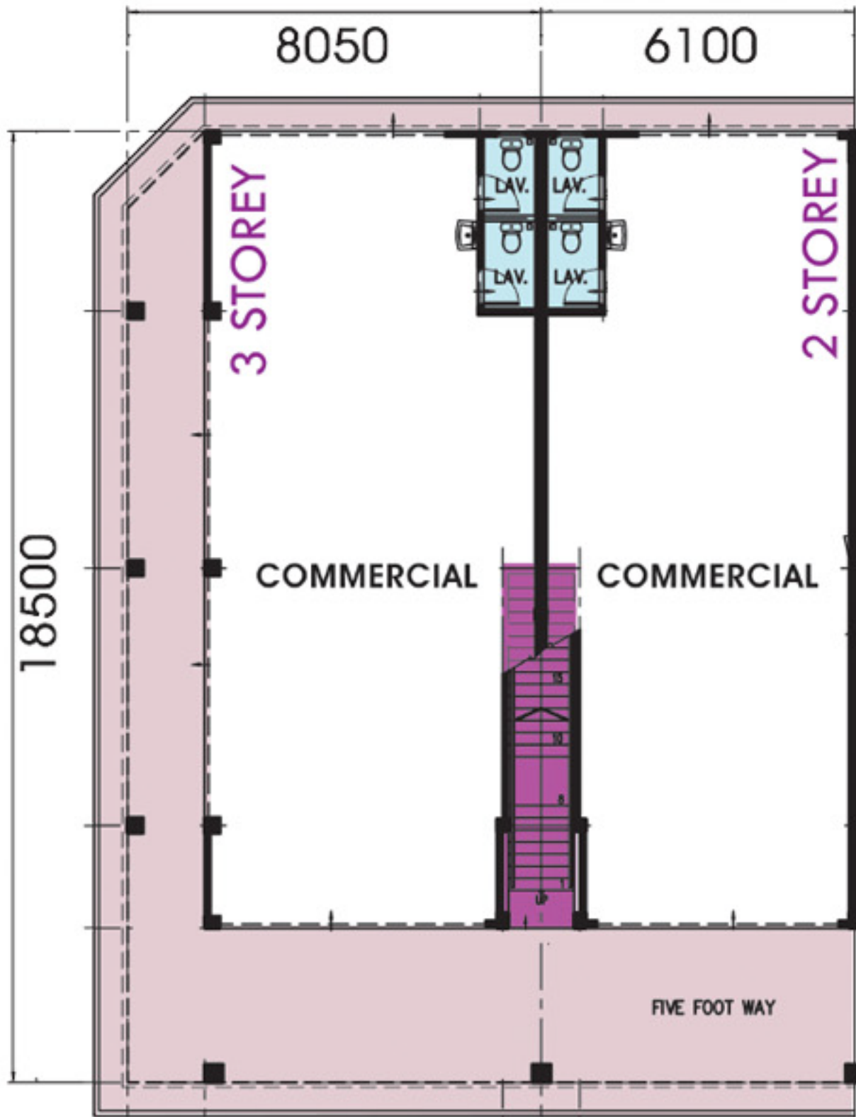
GROUND FLOOR
