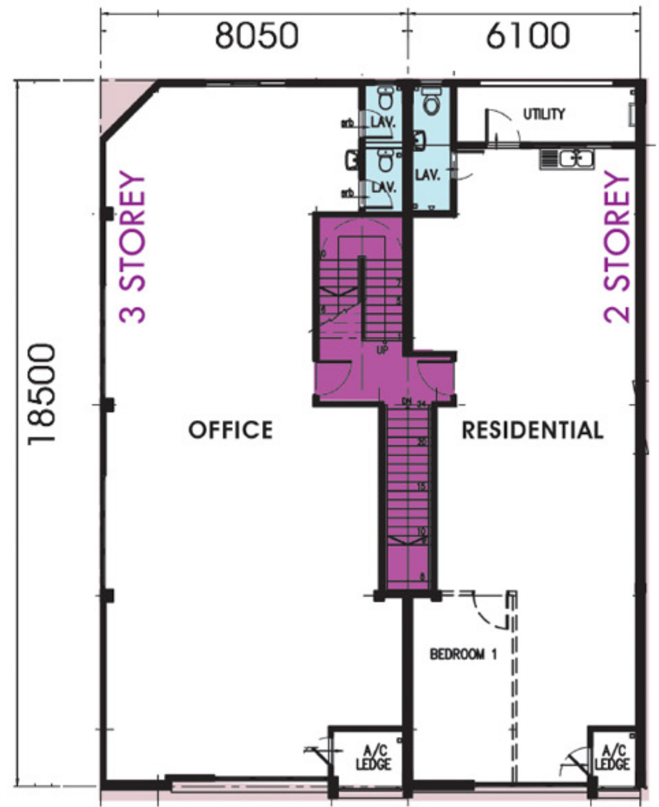
FIRST FLOOR
