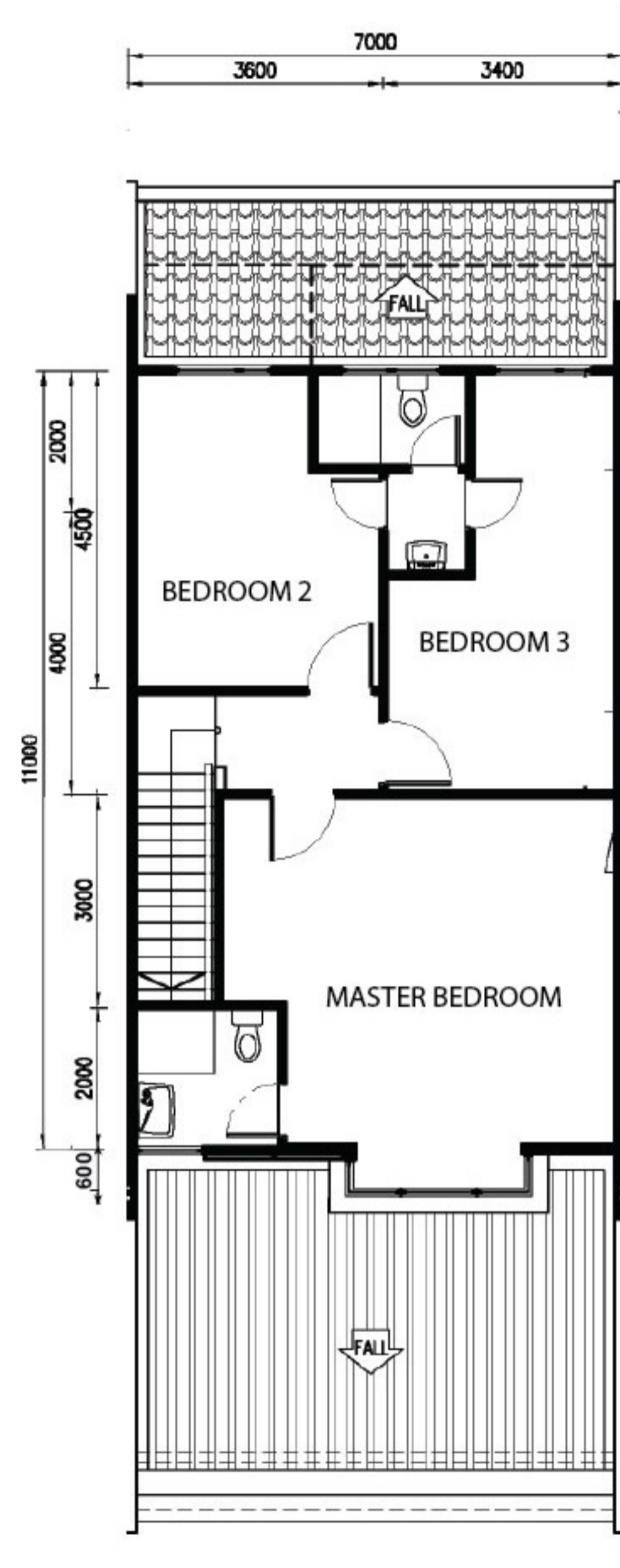
FIRST FLOOR
