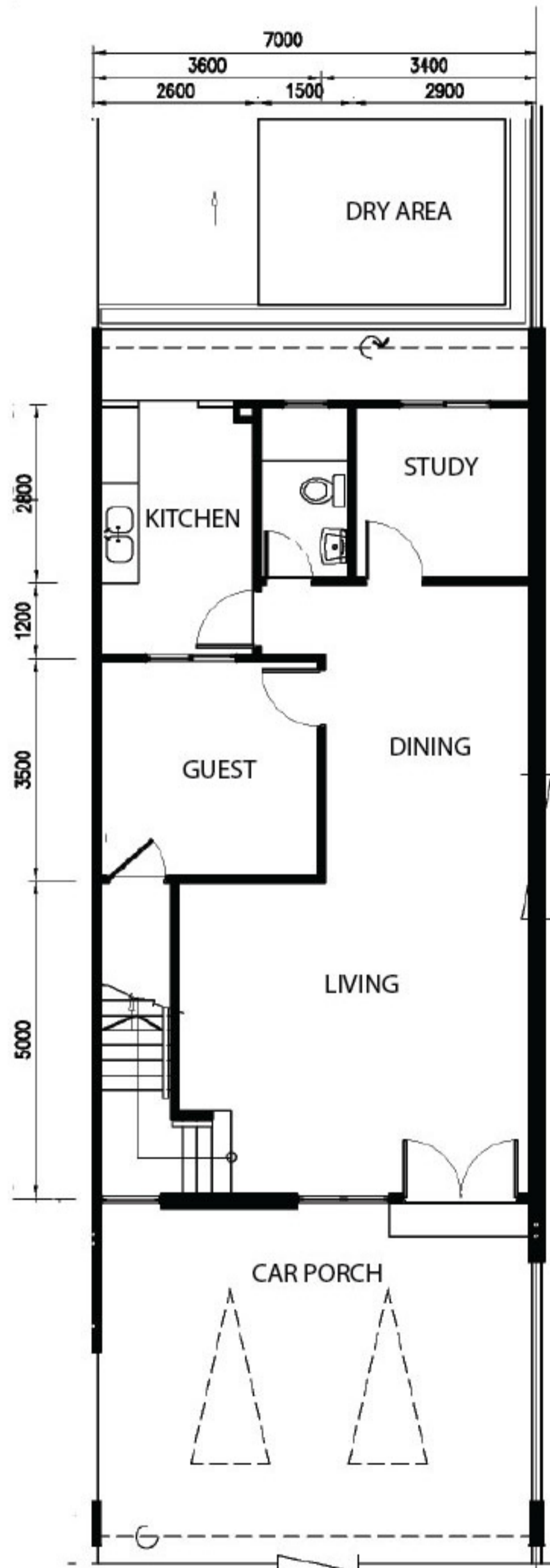
GROUND FLOOR
