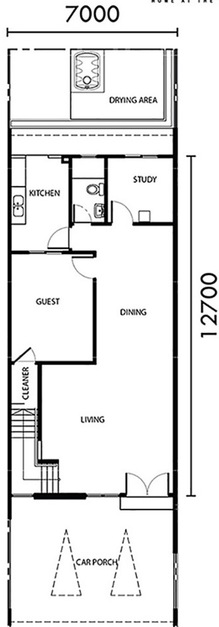
GROUND FLOOR
