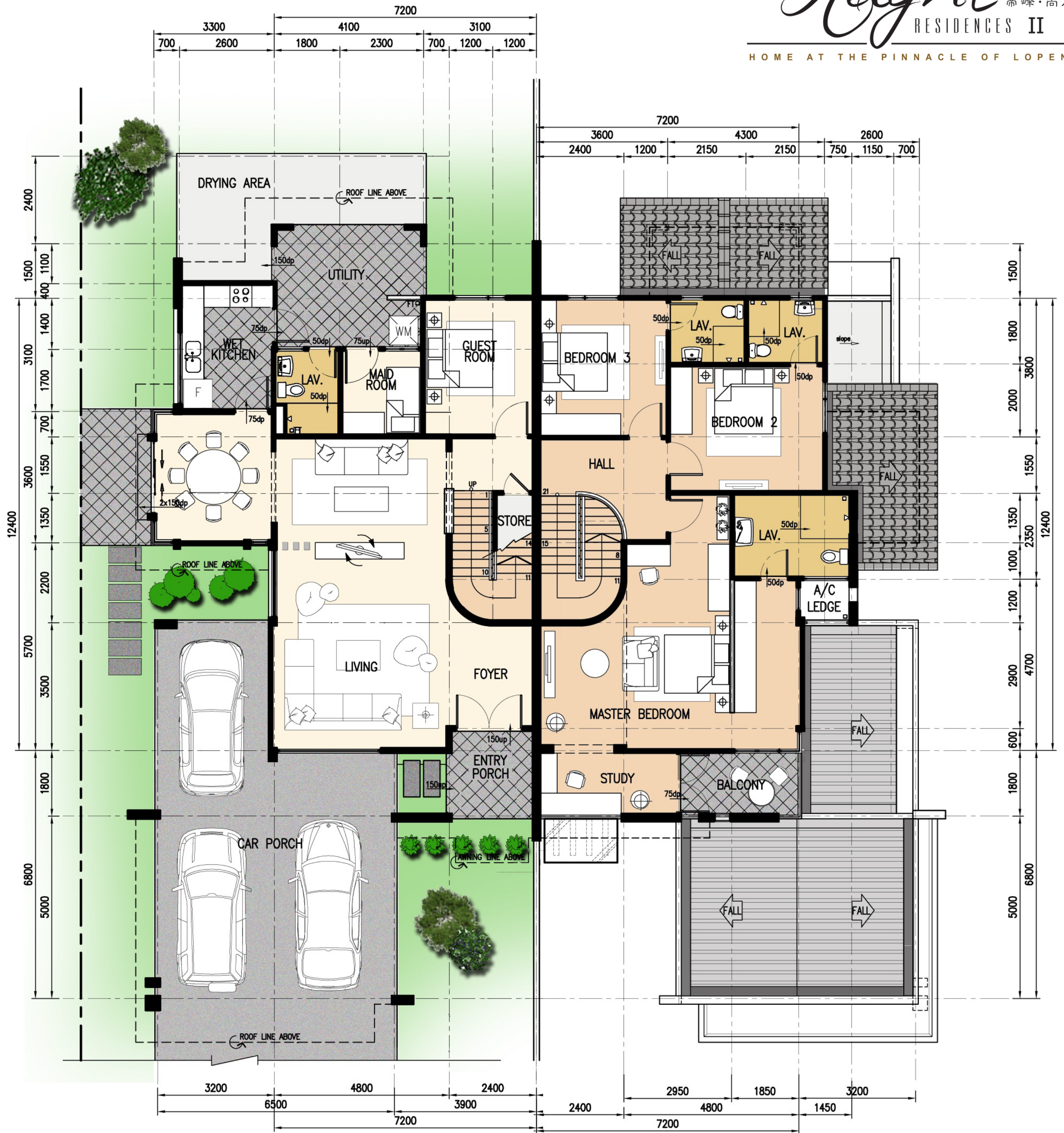
GROUND FLOOR
