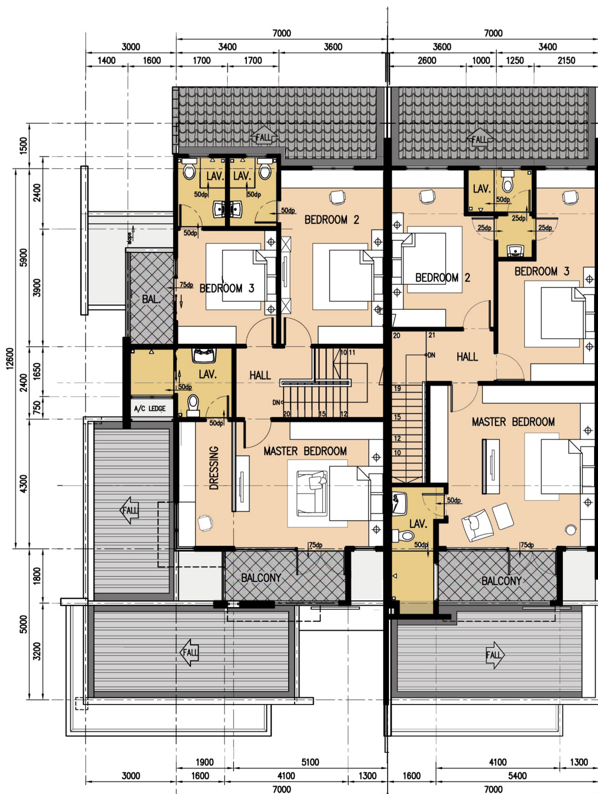
CORNER INTERMEDIATE FIRST FLOOR
