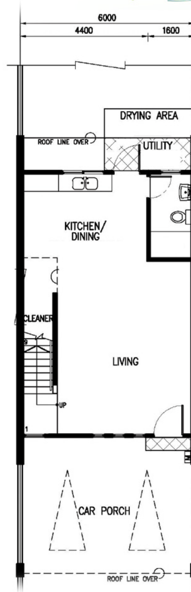
GROUND FLOOR
