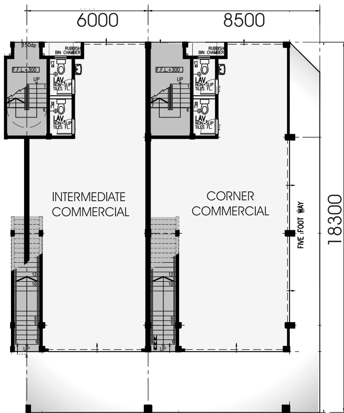
GROUND FLOOR
