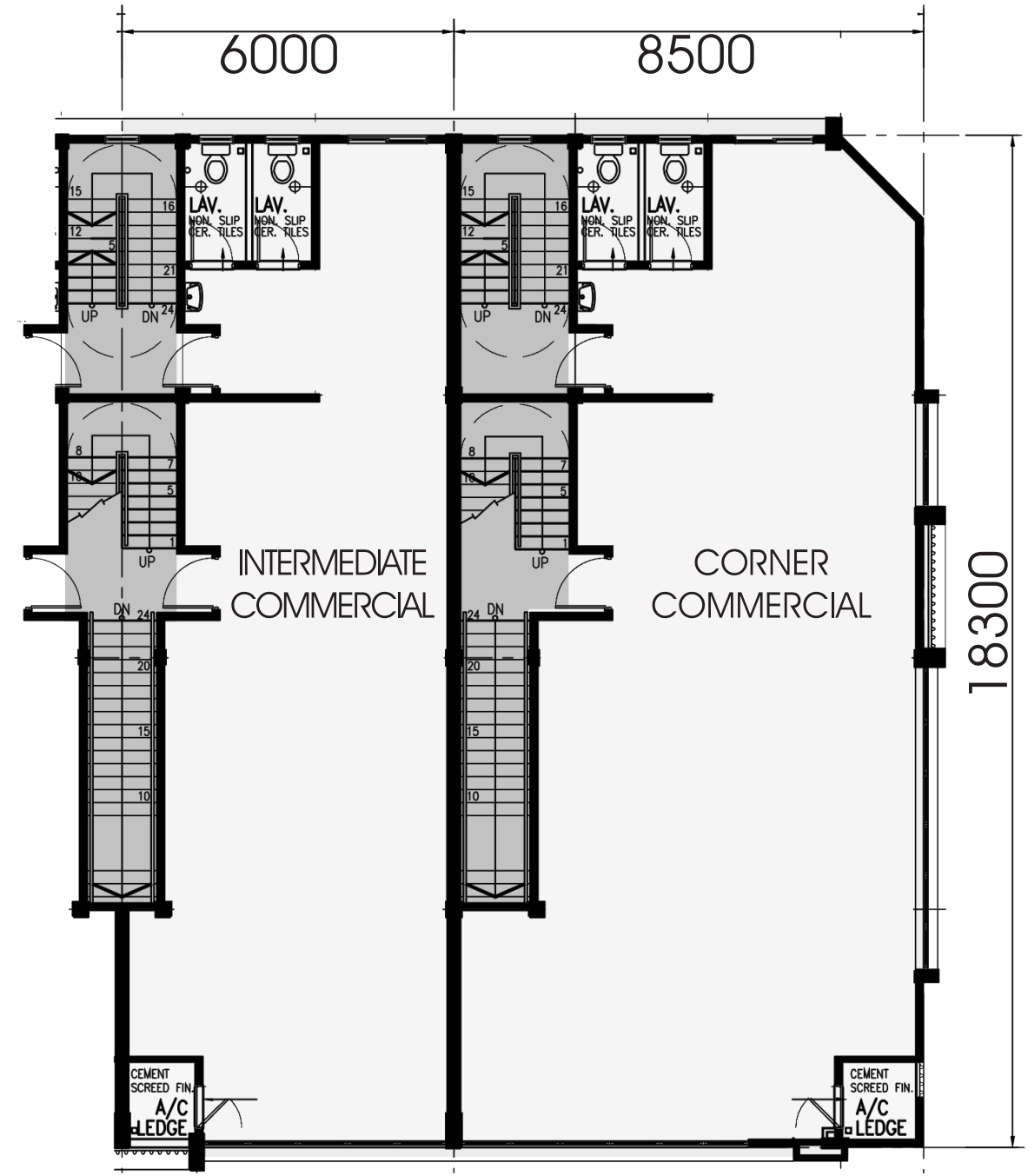
FIRST FLOOR
