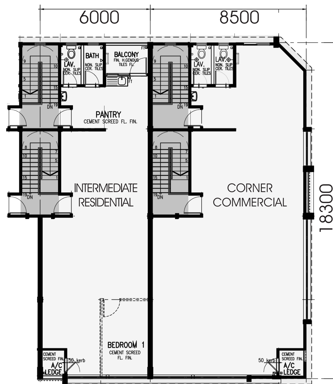
SECOND FLOOR
