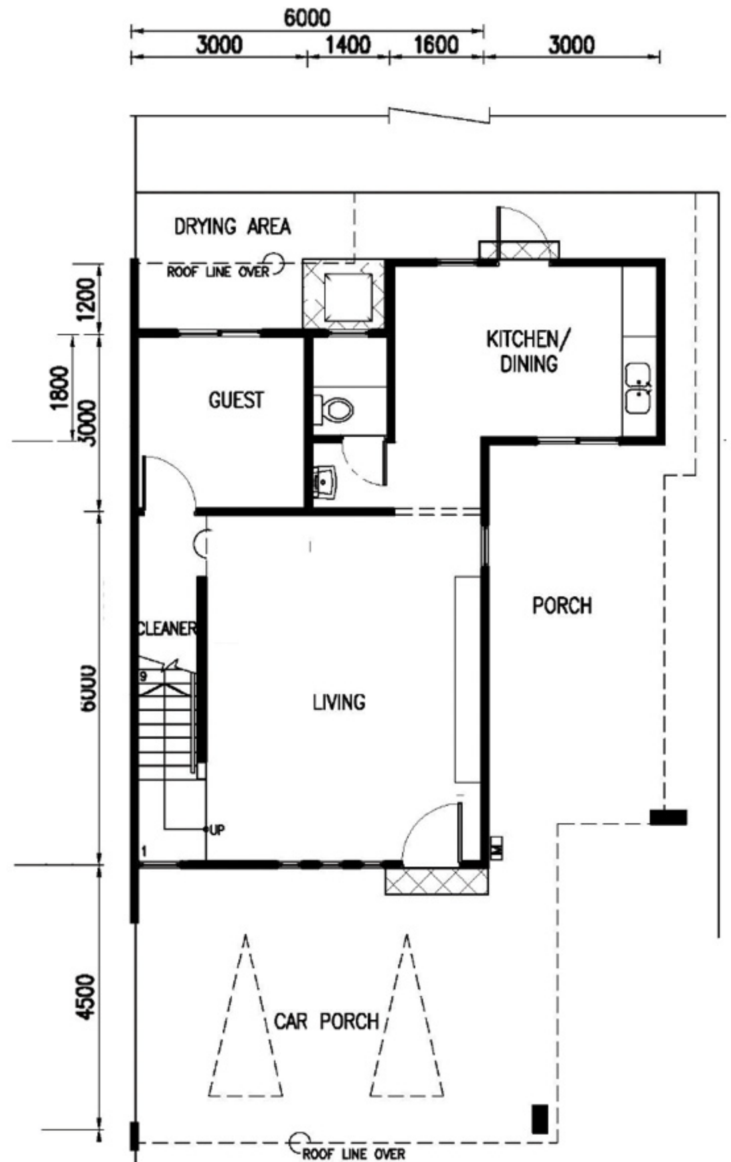
GROUND FLOOR
