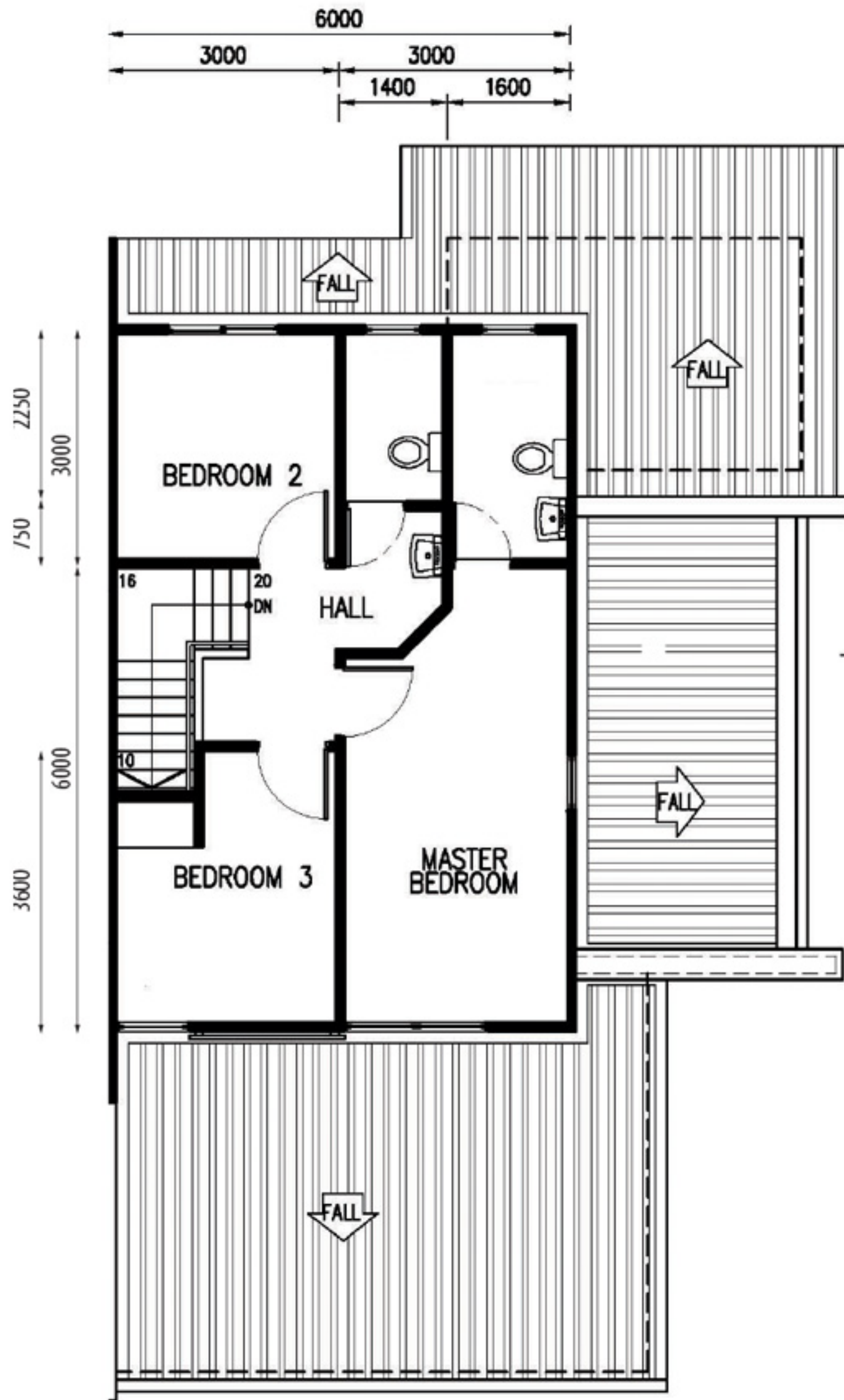
FIRST FLOOR
