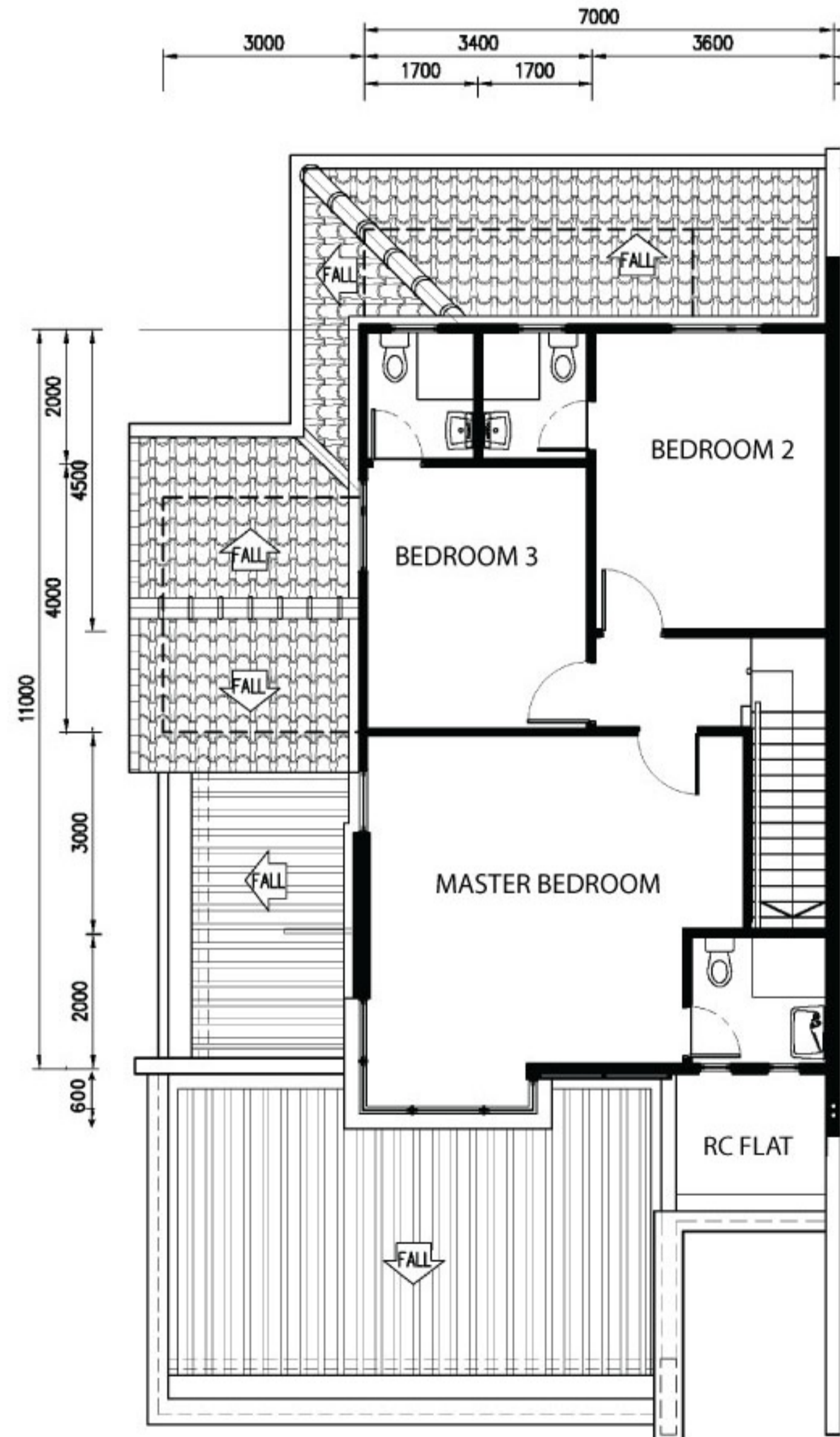
FIRST FLOOR
