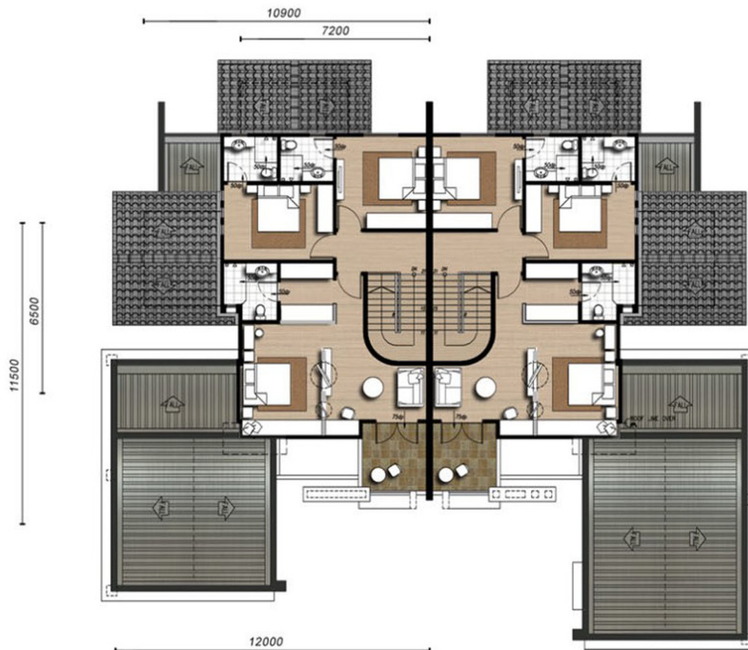
FIRST FLOOR
