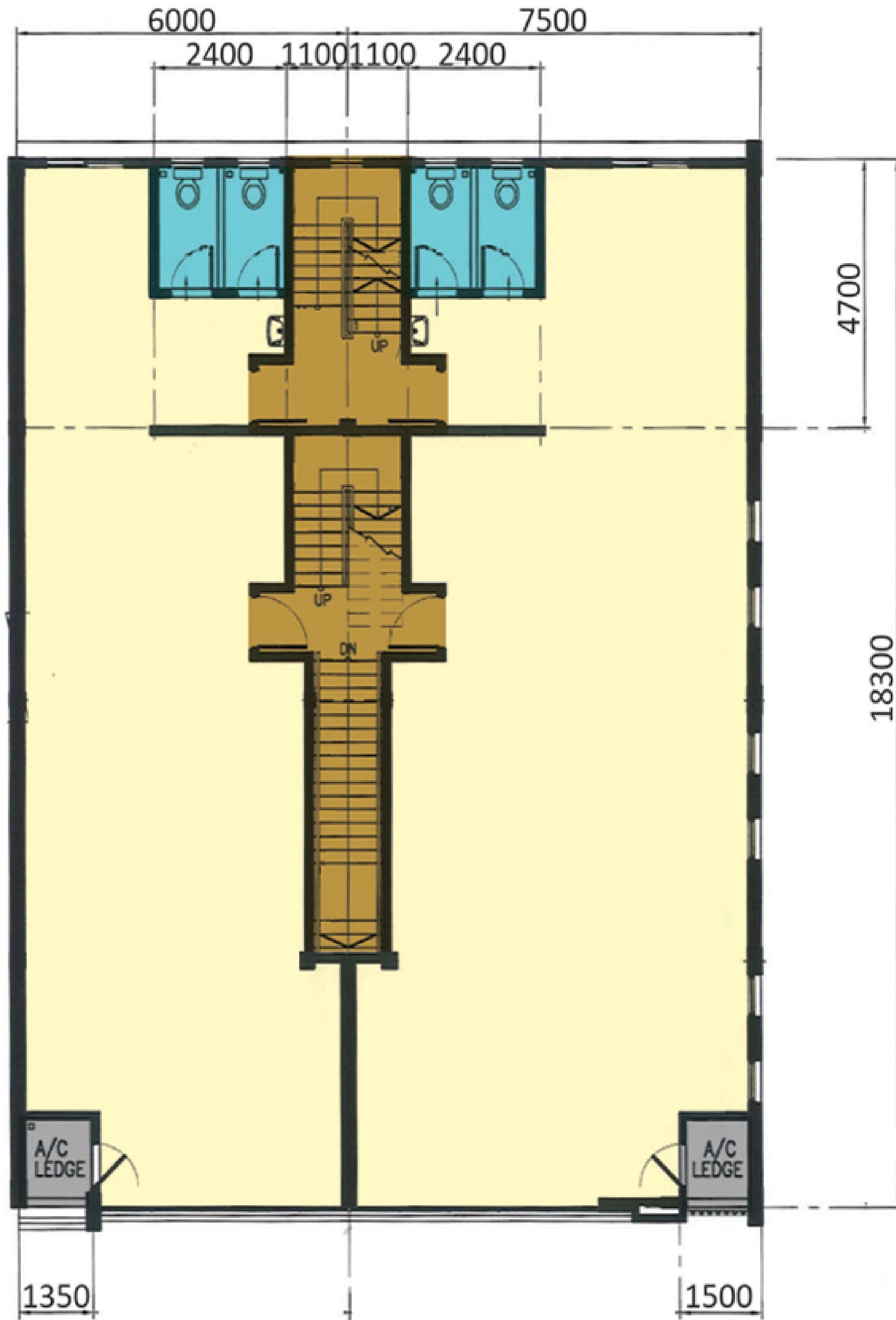
FIRST FLOOR
